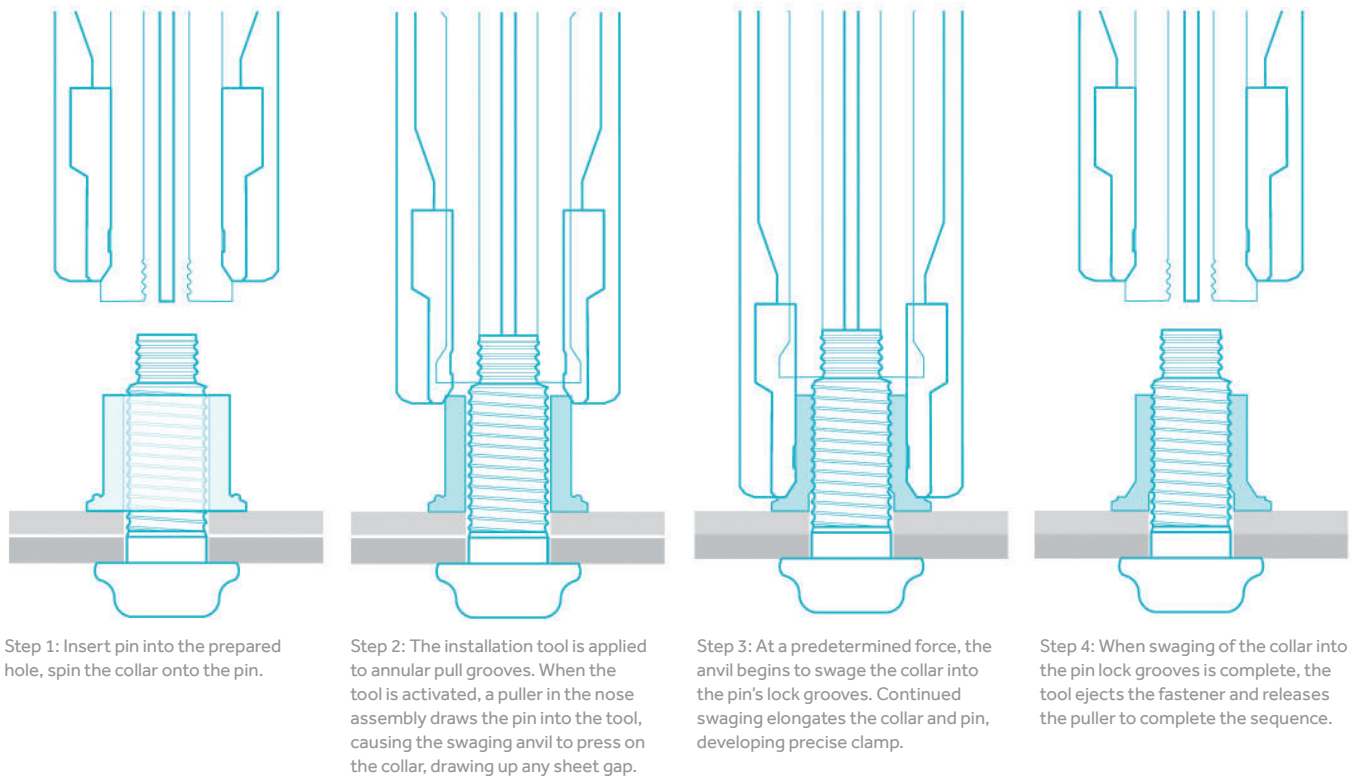
Figure 2: HuckBolt Installation Process
