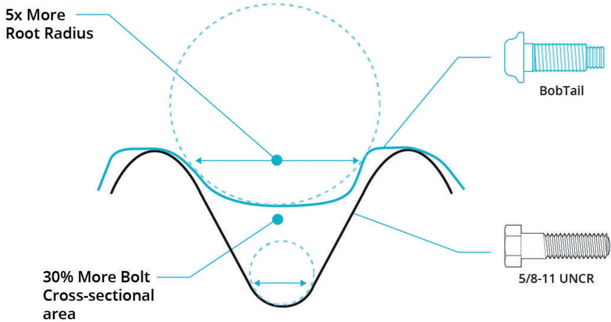
Figure 3: HuckBolt geometry optimization
