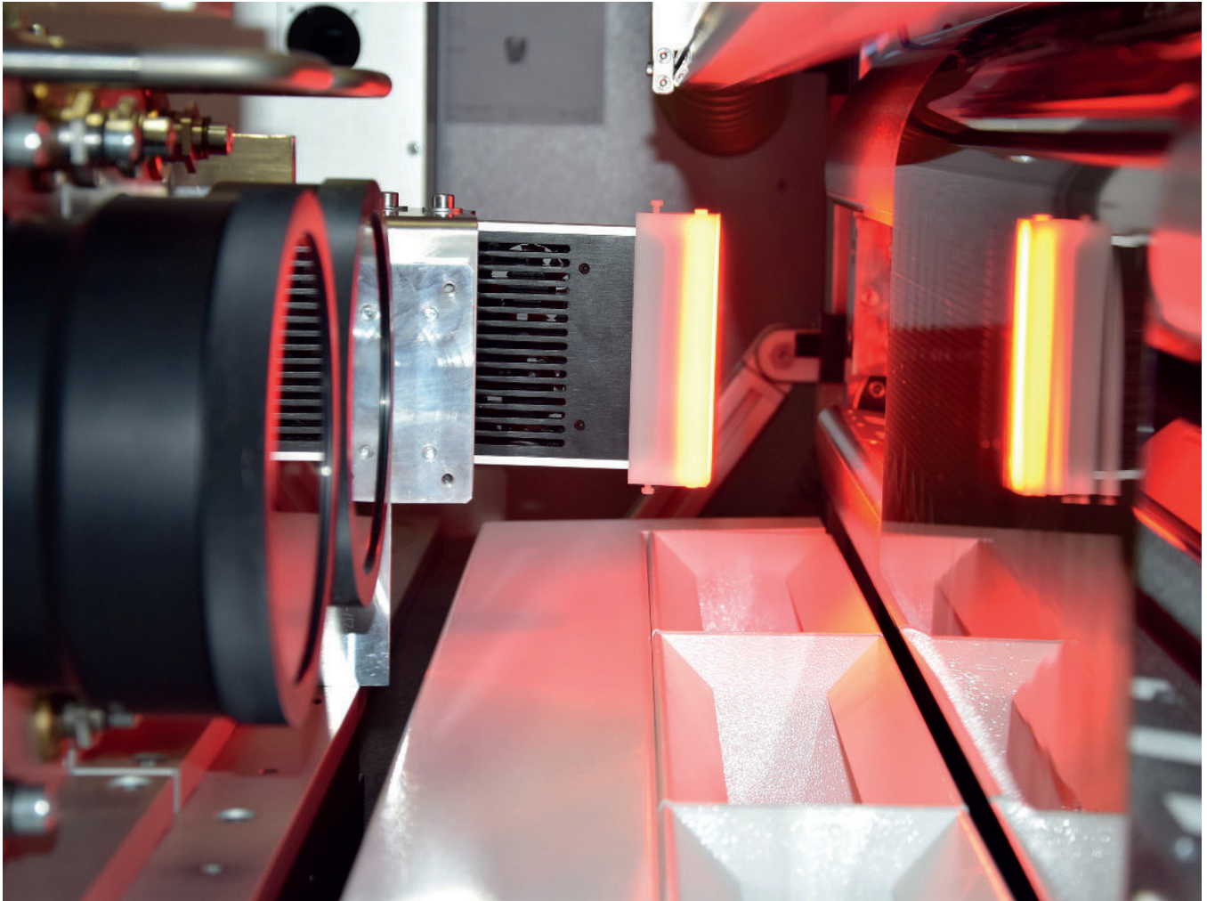
Fig 2. Transmitted light camera for the inspection of the thin film
