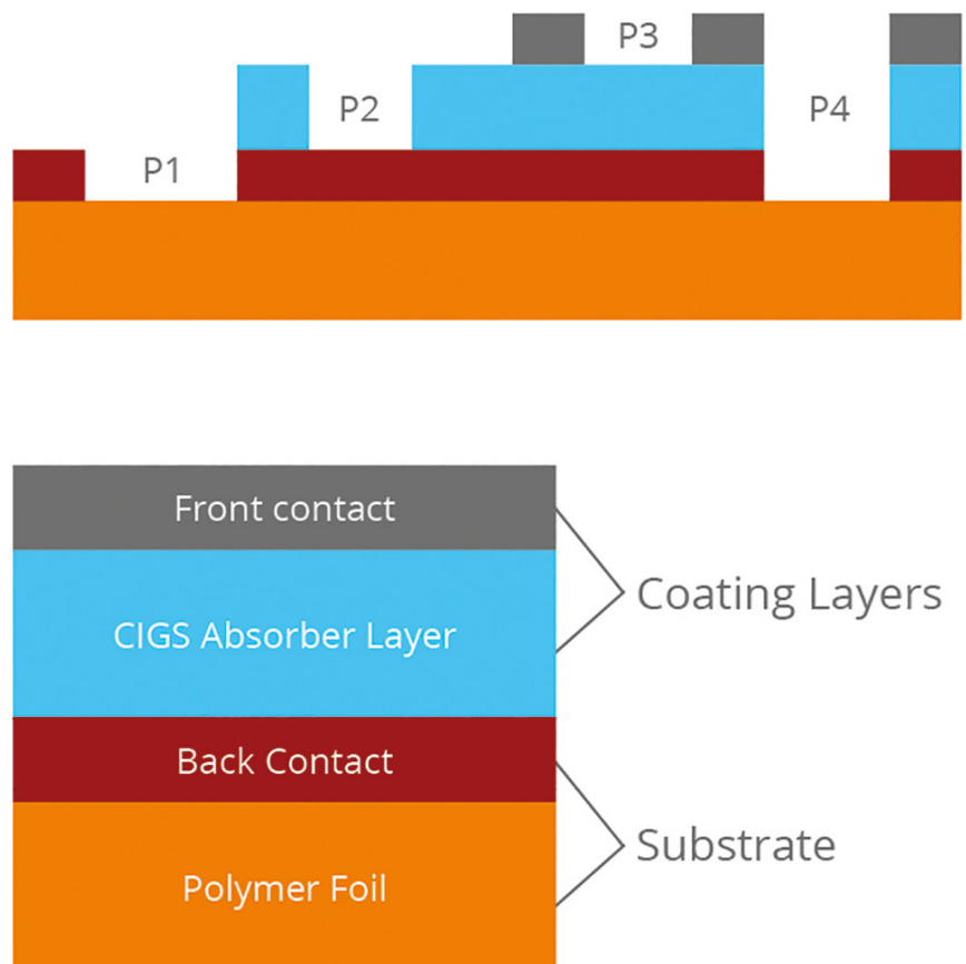
Fig. 1: Schematic of CIGS solar cell layers and laser scribes
