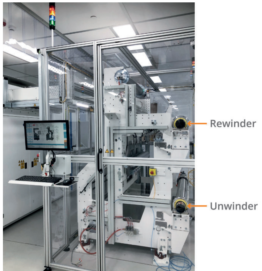
Fig. 4: Unwinder and rewinder are combined into one unit, allowing loading/unloading material from the same side; the integrated control panel is fully adjustable in angle and height
