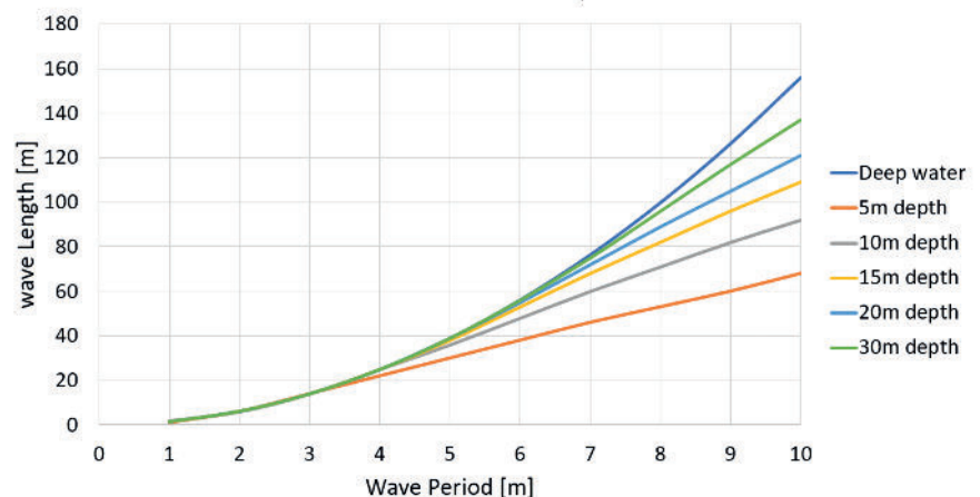
Wave Periods and Corresponding Wavelengths For Different Water Depths
